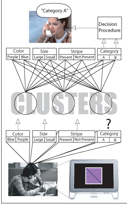
Figure 1: CLUSTER is an auto-associative learning model in which the hidden layer consists of clusters that adjust their position, attention, and association weights to minimize an error term that reflects the learner’s goals. In the illustrated example, three clusters have been recruited and the model is being asked to infer the category label.
